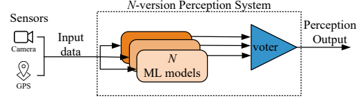
Figure 1: An example of an N-version perception system architecture, containing N ML models. ML models can assume one of the states in a given moment: healthy (H), compromised but operational (C), or non-operational (N).
